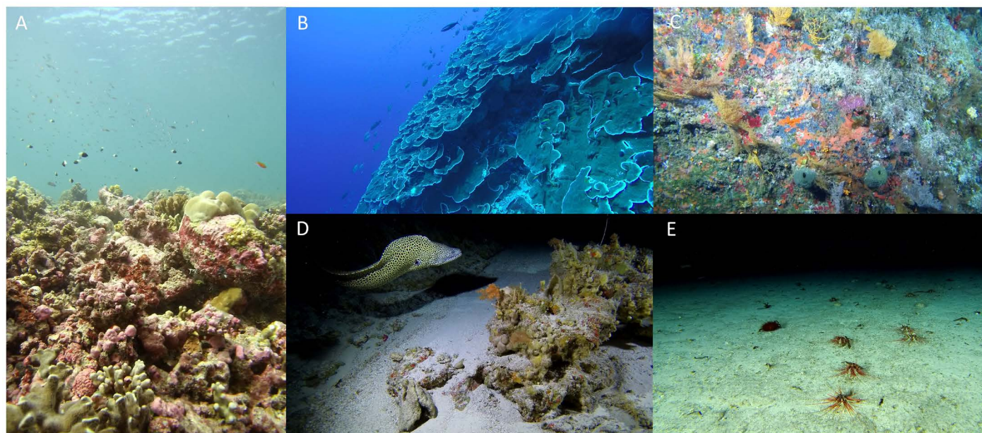
Fig. 4. A) Shallow-coral reefs teeming with life in Alphonse, 10 m, B) Incredible hard coral coverage and fish abundance at reefs in Astove, 30 m, C) Diverse benthic assemblages observed in Astove, 60 m, D) A moray eel spotted in Aldabra, 120 m, E) Sea urchins populating the deeper sedimented habitats in Desroches, 250 m © Nekton.
