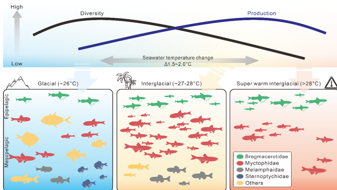
Fig. 2. Linkage of deep-sea fish abundance and diversity and seawater temperature on glacial/interglacial time scales.
